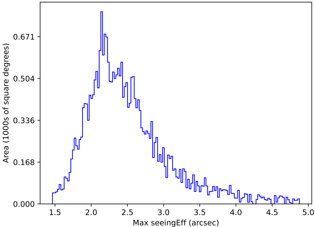
noroll_mjdp270_v3.4_10yrs All sky i band: Max seeingEff
