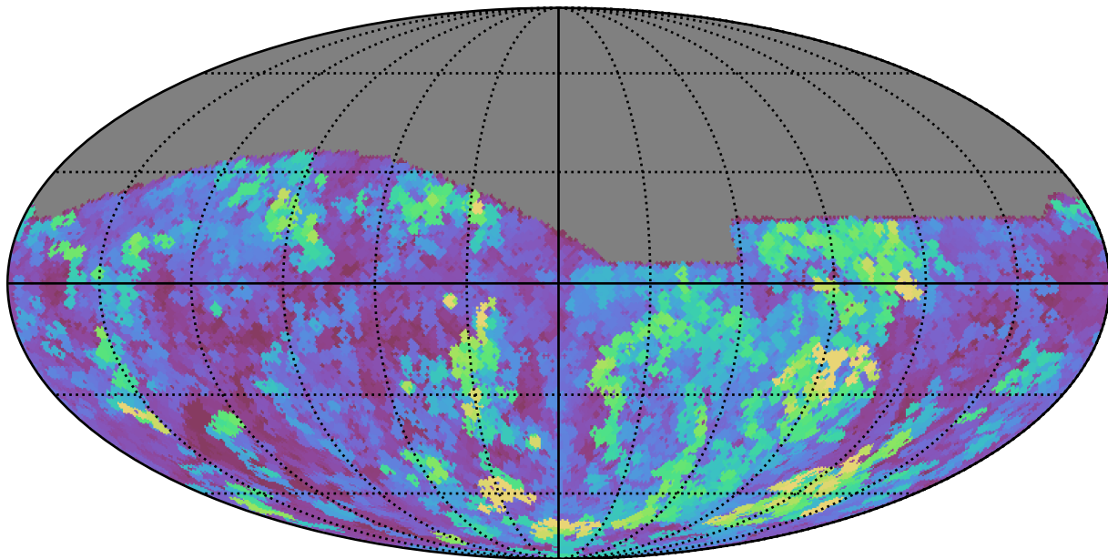
noroll_mjdp270_v3.4_10yrs All sky g band: Max seeingEff
