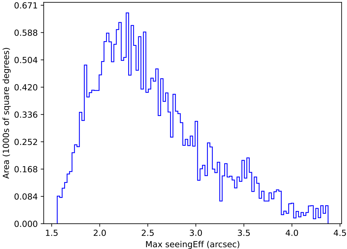
noroll_mjdp270_v3.4_10yrs All sky g band: Max seeingEff
