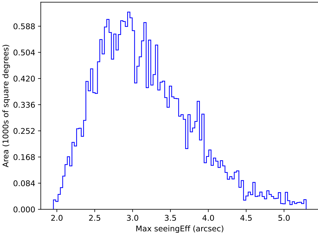
noroll_mjdp270_v3.4_10yrs All sky all bands: Max seeingEff
