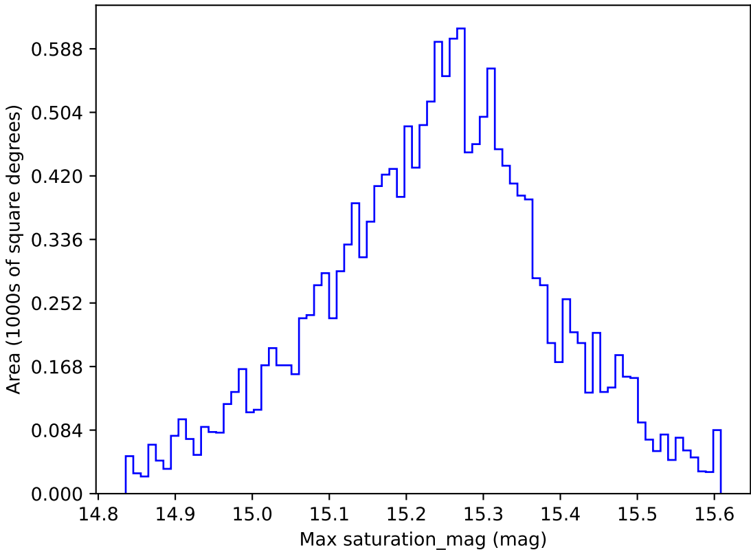
noroll_mjdp270_v3.4_10yrs WFD z band: Max saturation_mag
