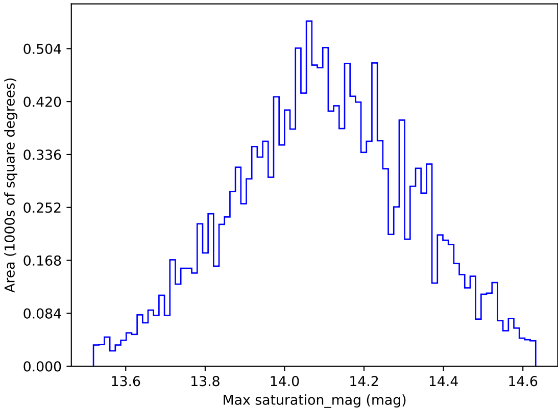
noroll_mjdp270_v3.4_10yrs WFD u band: Max saturation_mag
