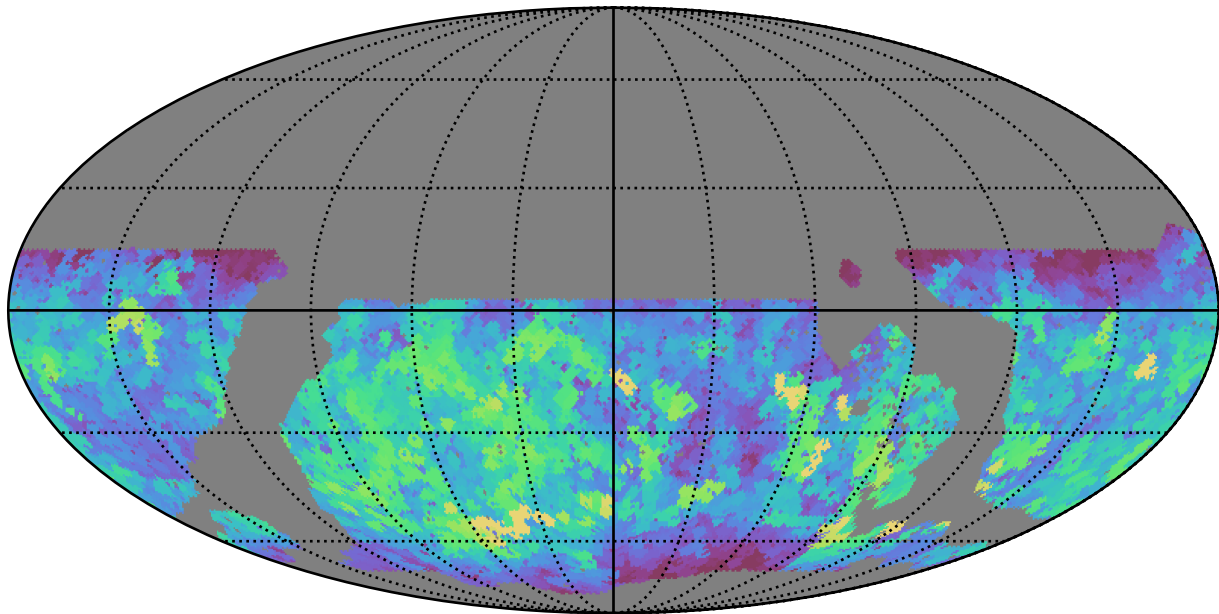
noroll_mjdp270_v3.4_10yrs WFD r band: Max saturation_mag
