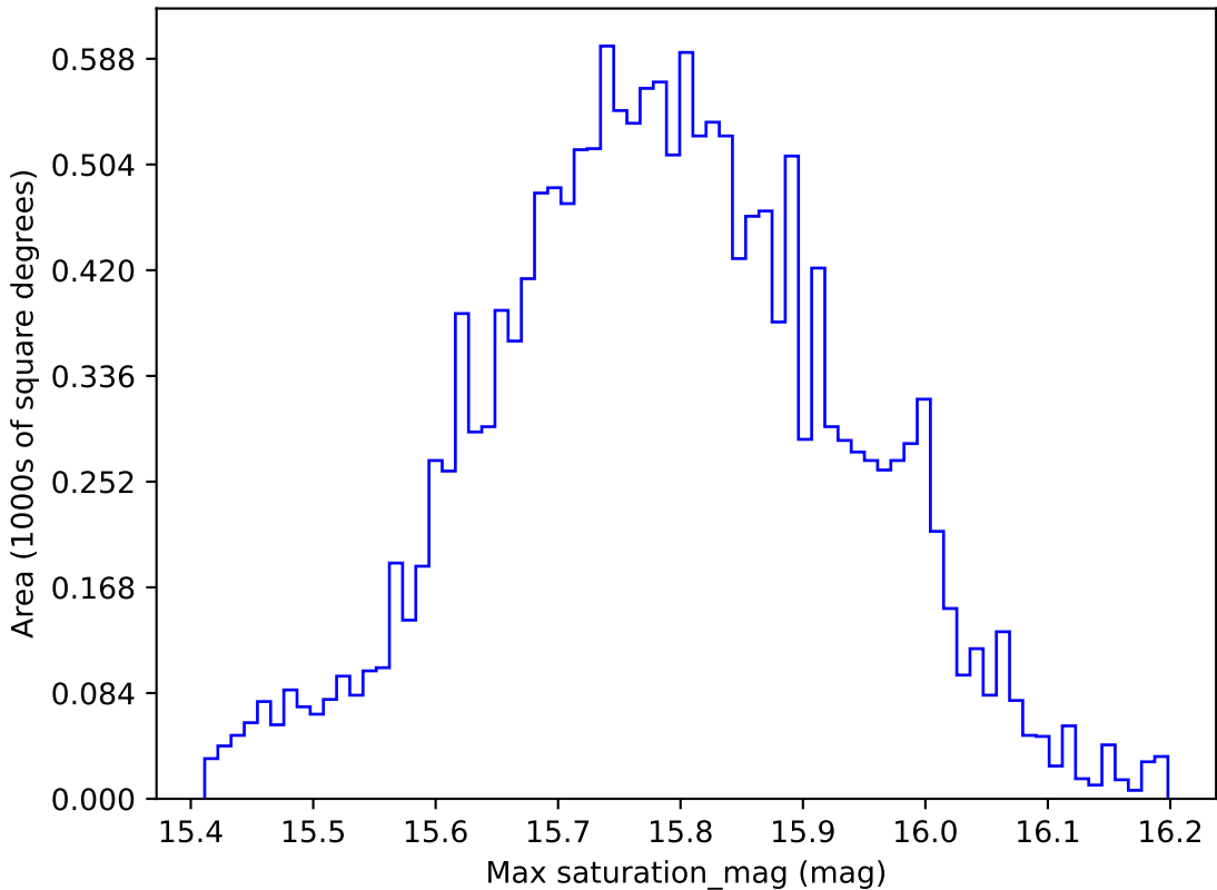
noroll_mjdp270_v3.4_10yrs WFD r band: Max saturation_mag
