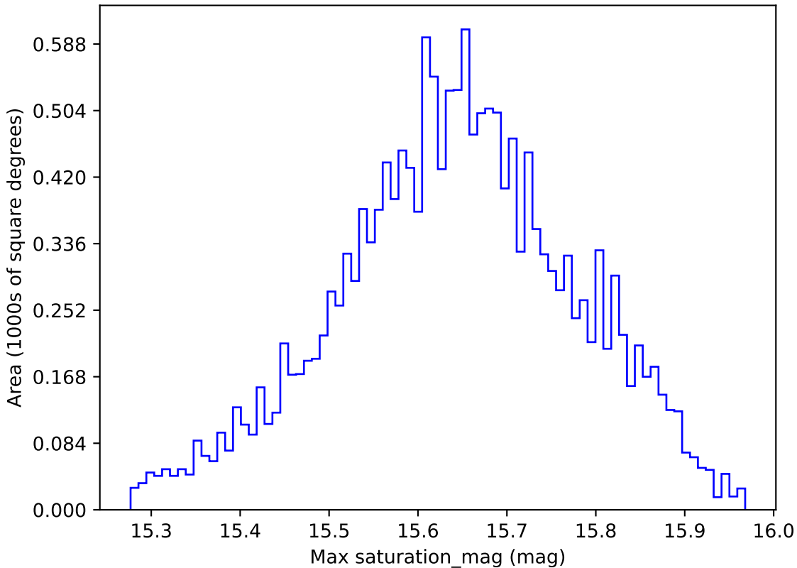
noroll_mjdp270_v3.4_10yrs WFD i band: Max saturation_mag
