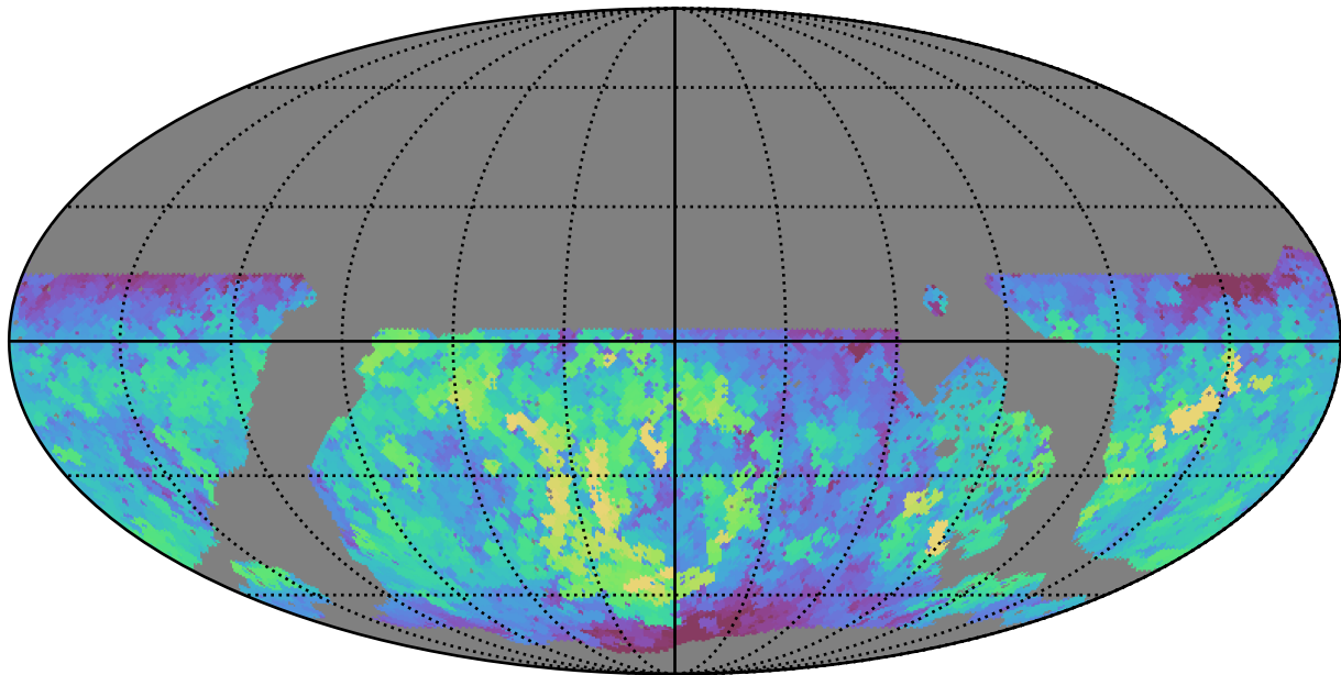
noroll_mjdp270_v3.4_10yrs WFD g band: Max saturation_mag
