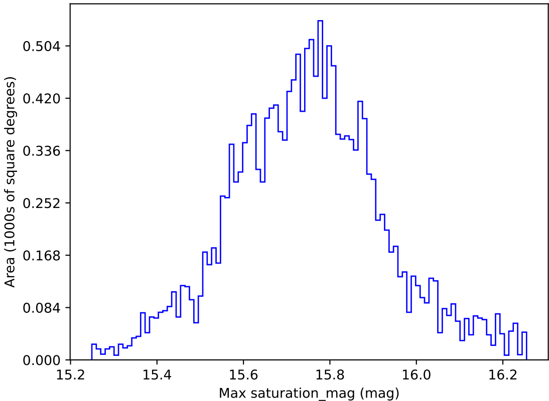
noroll_mjdp270_v3.4_10yrs WFD g band: Max saturation_mag
