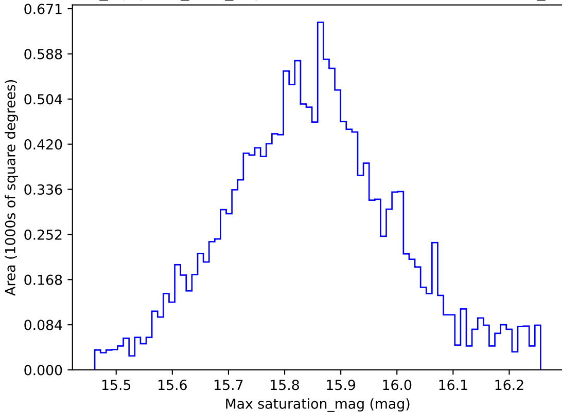
noroll_mjdp270_v3.4_10yrs WFD all bands: Max saturation_mag
