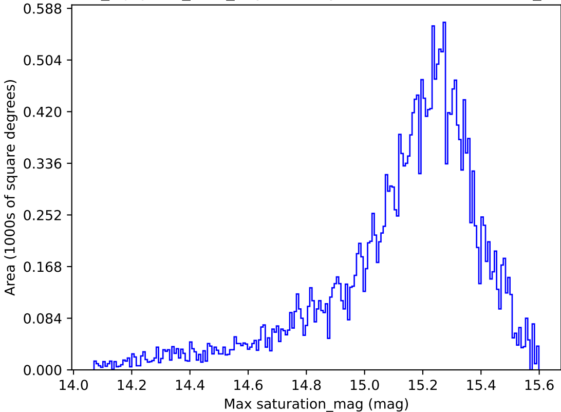
noroll_mjdp270_v3.4_10yrs All sky z band: Max saturation_mag
