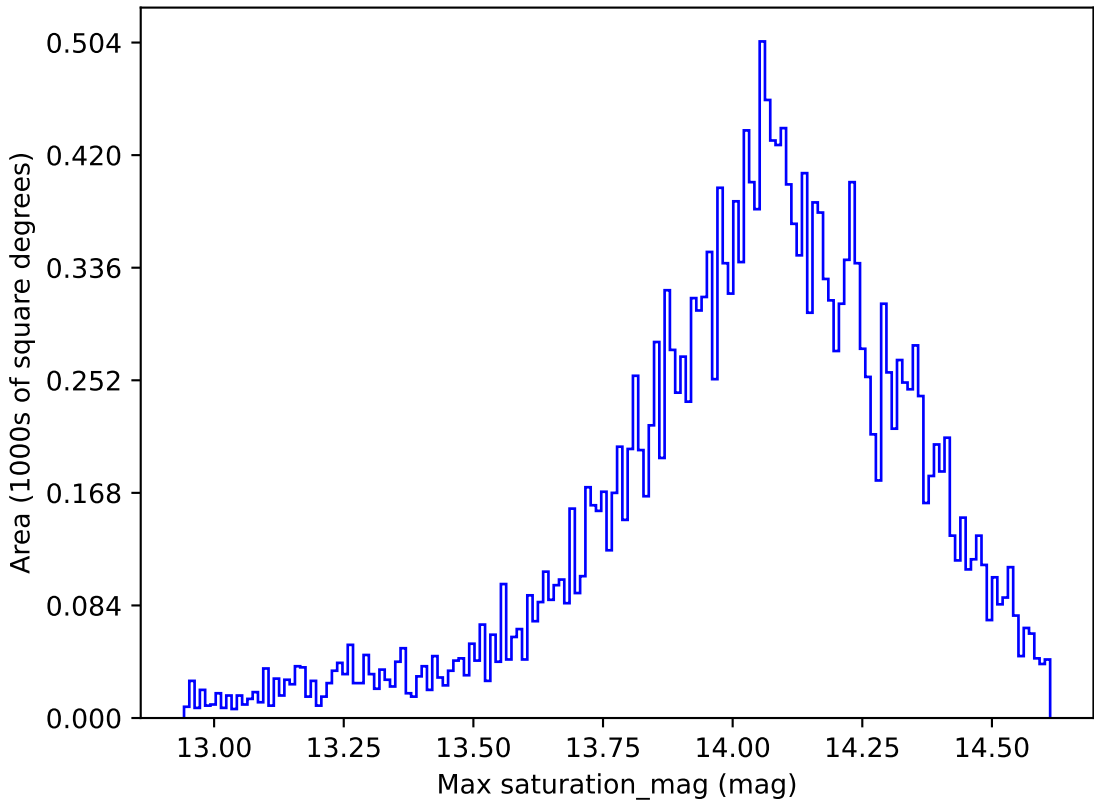
noroll_mjdp270_v3.4_10yrs All sky u band: Max saturation_mag
