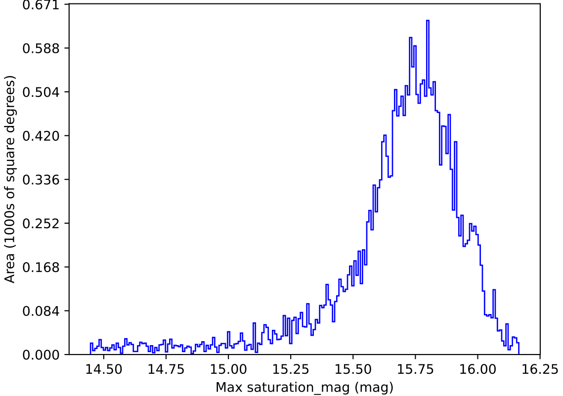
noroll_mjdp270_v3.4_10yrs All sky r band: Max saturation_mag
