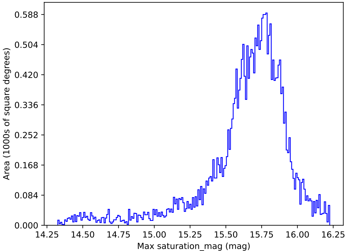
noroll_mjdp270_v3.4_10yrs All sky g band: Max saturation_mag
