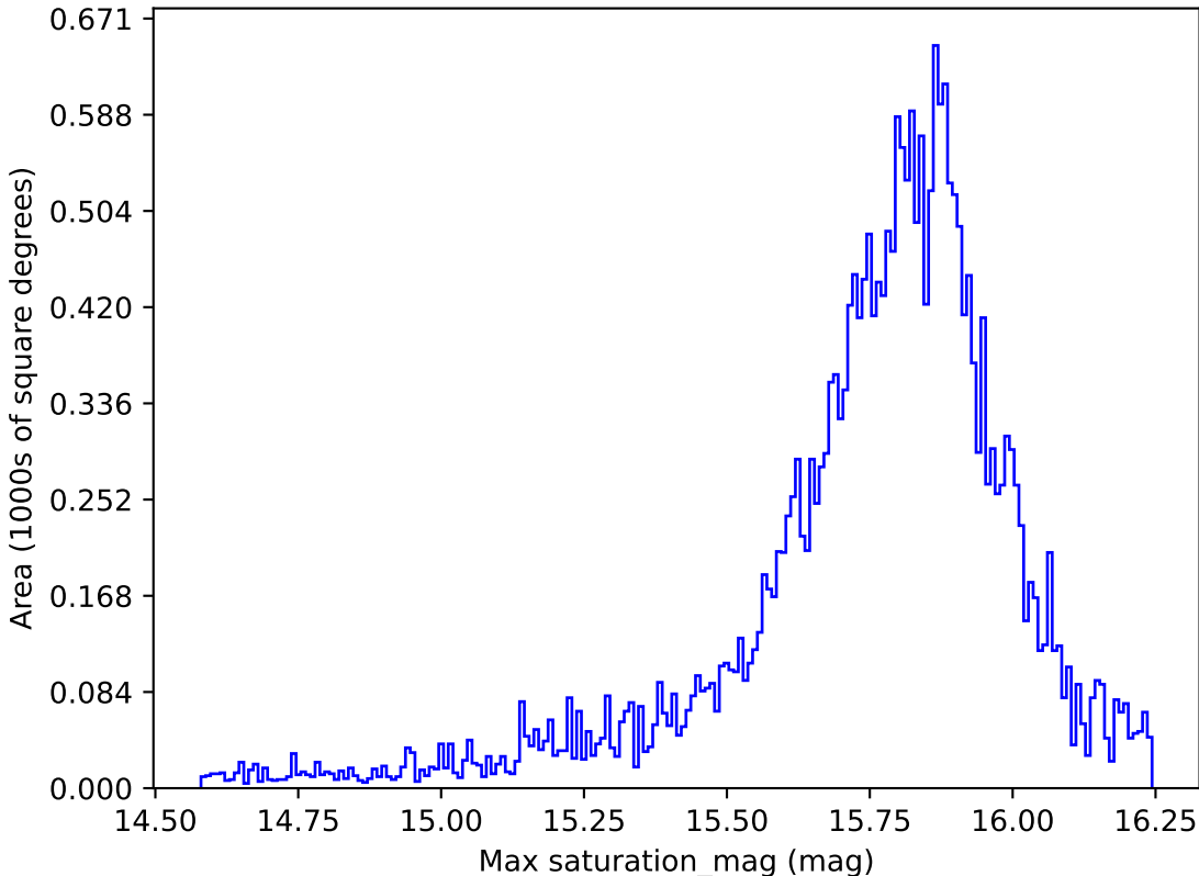
noroll_mjdp270_v3.4_10yrs All sky all bands: Max saturation_mag
