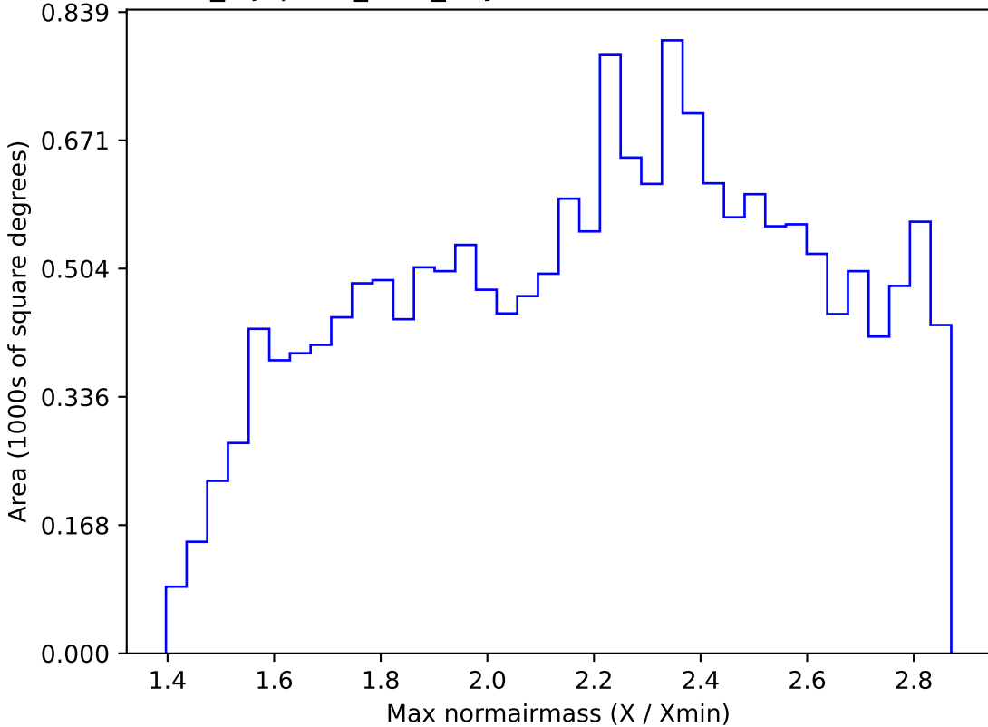
noroll_mjdp270_v3.4_10yrs WFD z band: Max normairmass
