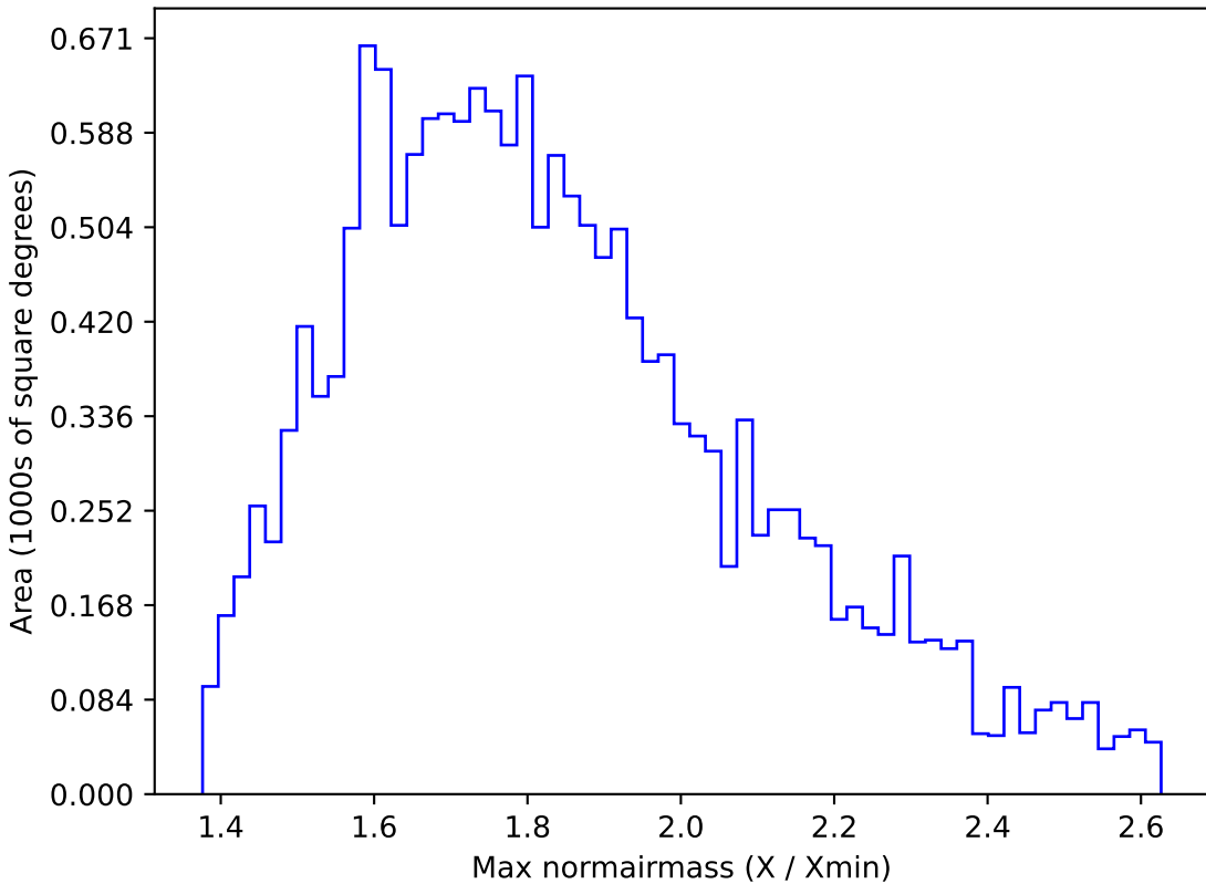
noroll_mjdp270_v3.4_10yrs WFD y band: Max normairmass
