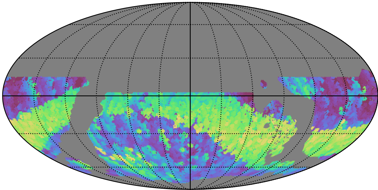
noroll_mjdp270_v3.4_10yrs WFD r band: Max normairmass
