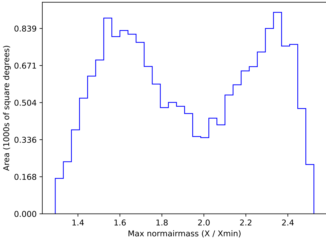
noroll_mjdp270_v3.4_10yrs WFD r band: Max normairmass
