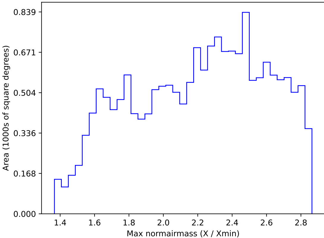
noroll_mjdp270_v3.4_10yrs WFD i band: Max normairmass
