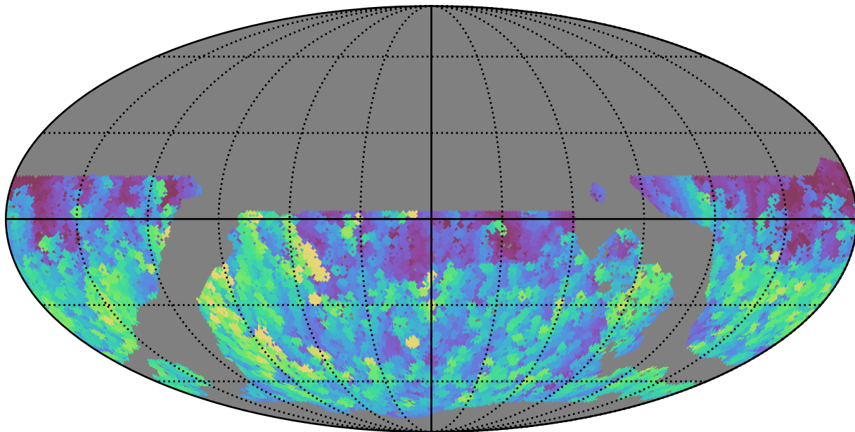
noroll_mjdp270_v3.4_10yrs WFD g band: Max normairmass
