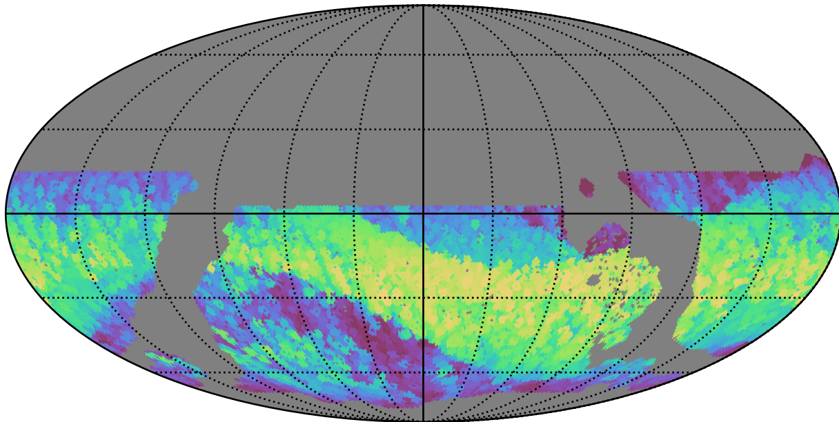
noroll_mjdp270_v3.4_10yrs WFD all bands: Max normairmass
