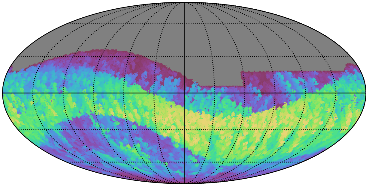
noroll_mjdp270_v3.4_10yrs All sky z band: Max normairmass
