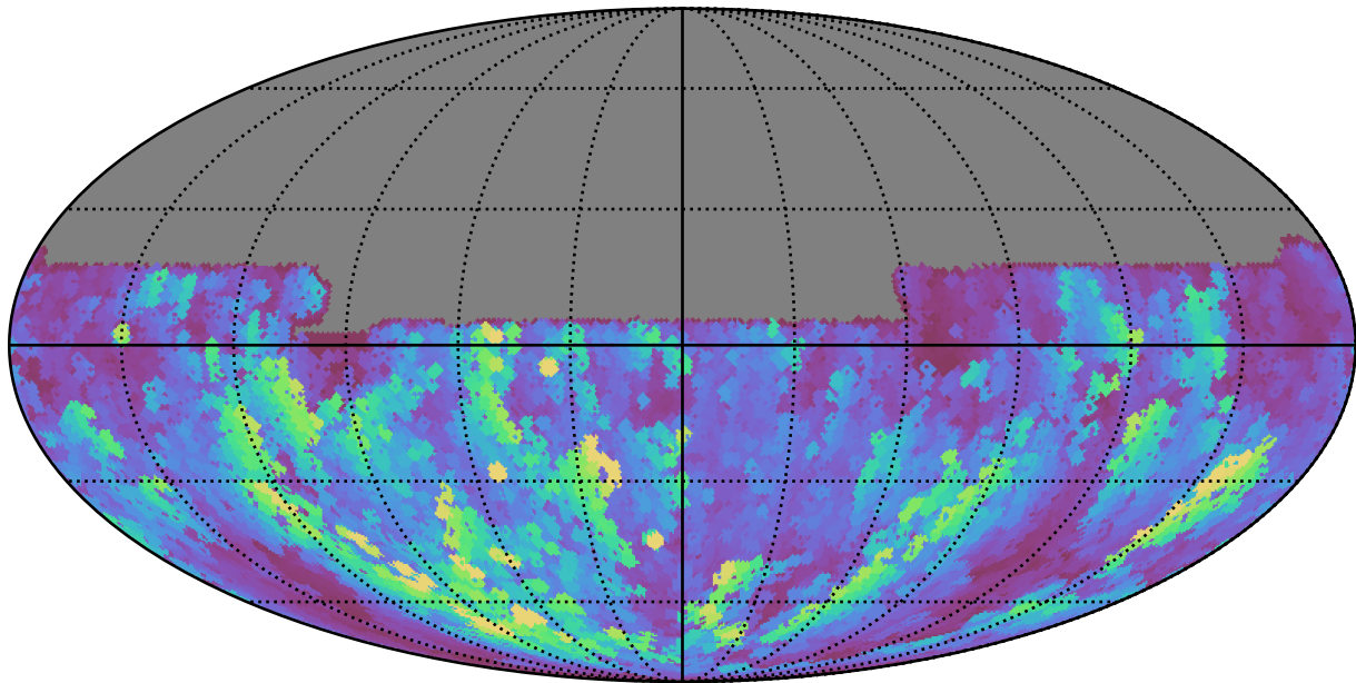
noroll_mjdp270_v3.4_10yrs All sky u band: Max normairmass
