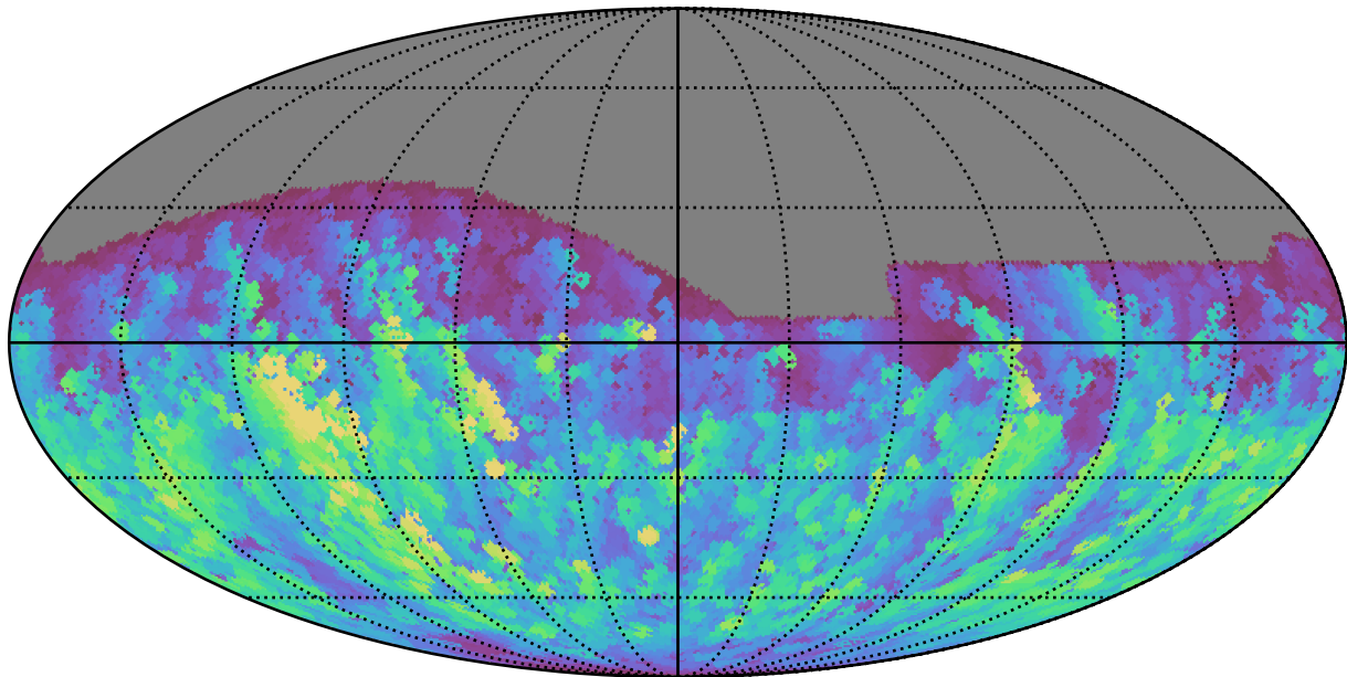
noroll_mjdp270_v3.4_10yrs All sky g band: Max normairmass
