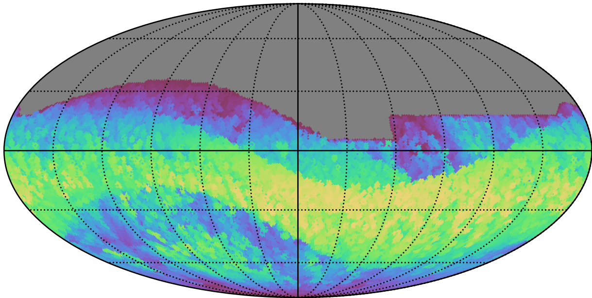
noroll_mjdp270_v3.4_10yrs All sky all bands: Max normairmass
