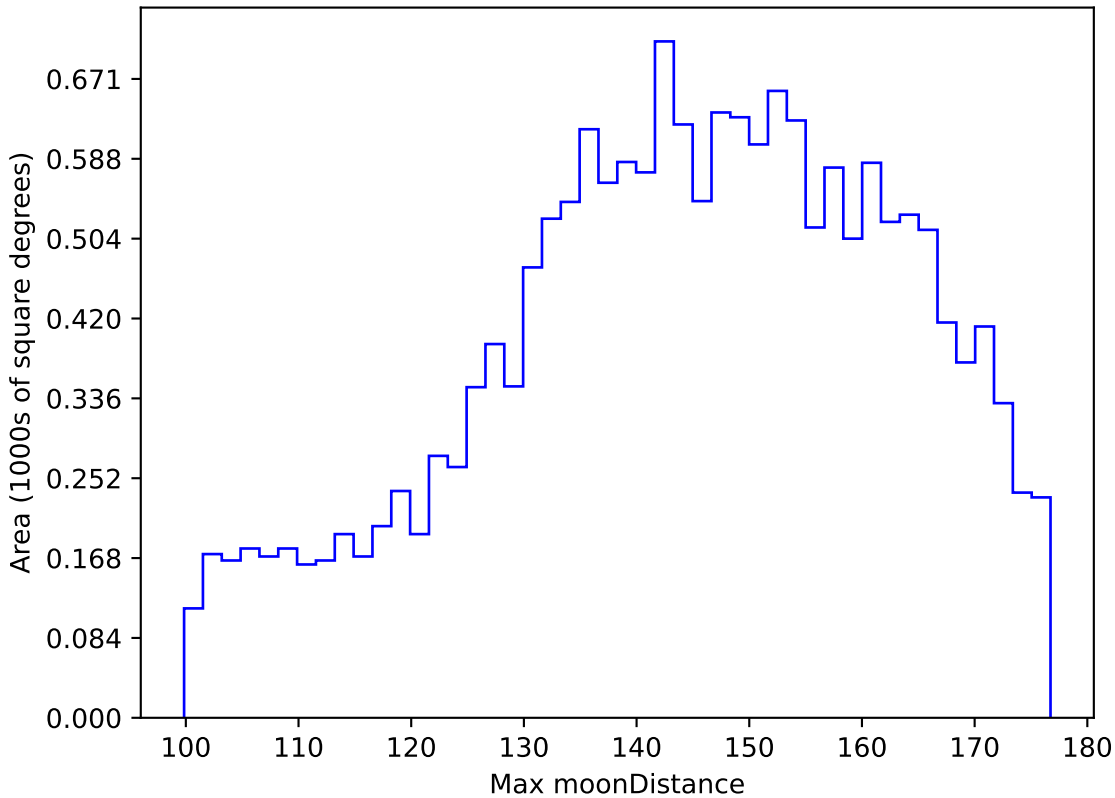
noroll_mjdp270_v3.4_10yrs WFD y band: Max moonDistance
