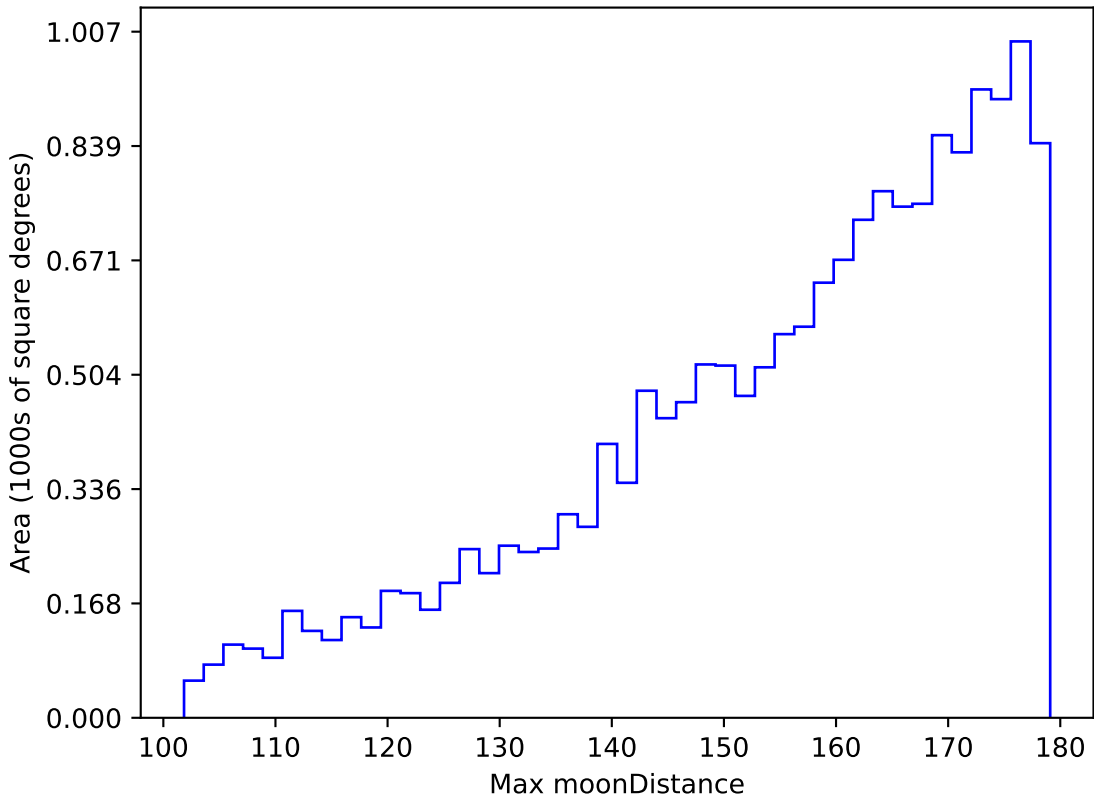
noroll_mjdp270_v3.4_10yrs WFD u band: Max moonDistance
