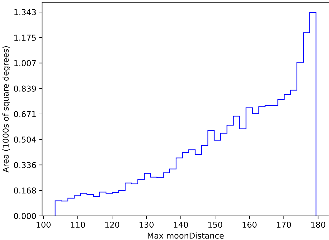
noroll_mjdp270_v3.4_10yrs WFD i band: Max moonDistance
