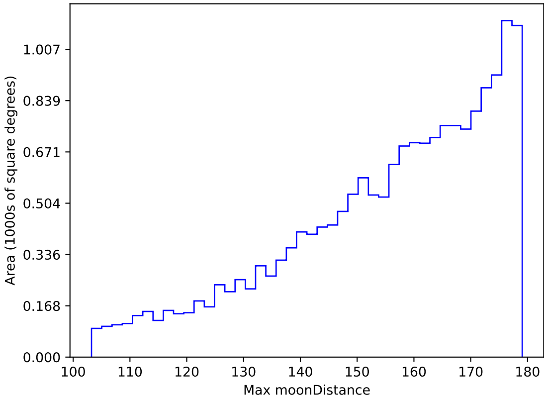
noroll_mjdp270_v3.4_10yrs WFD g band: Max moonDistance
