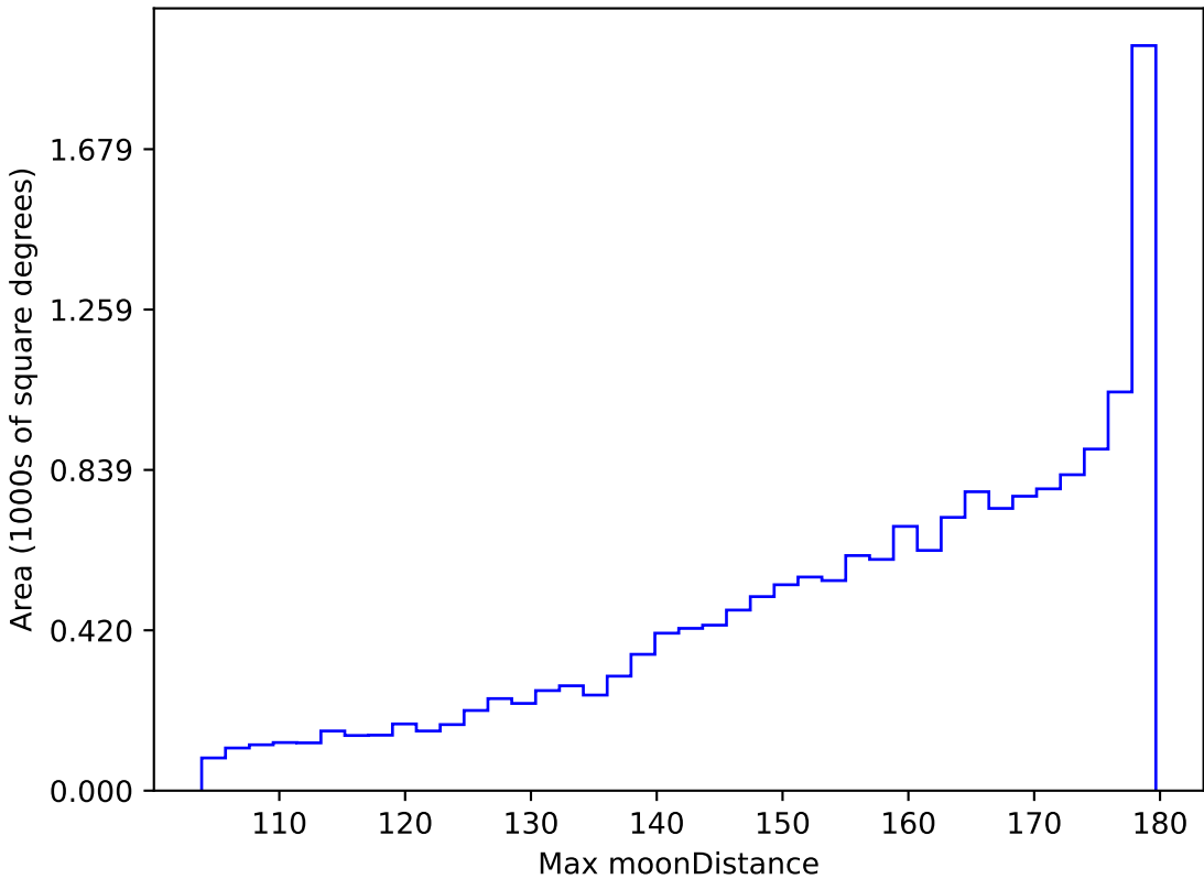
noroll_mjdp270_v3.4_10yrs WFD all bands: Max moonDistance
