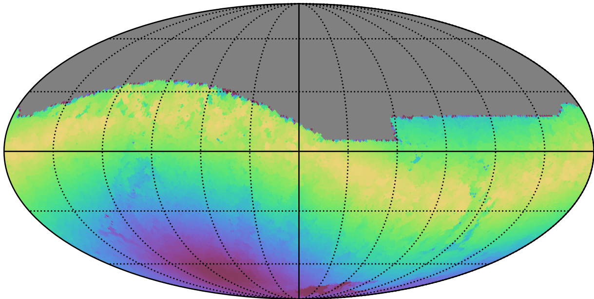
noroll_mjdp270_v3.4_10yrs All sky z band: Max moonDistance
