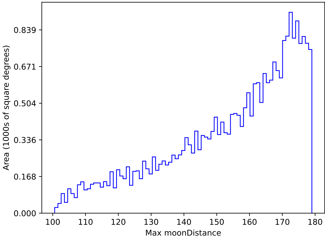
noroll_mjdp270_v3.4_10yrs All sky z band: Max moonDistance
