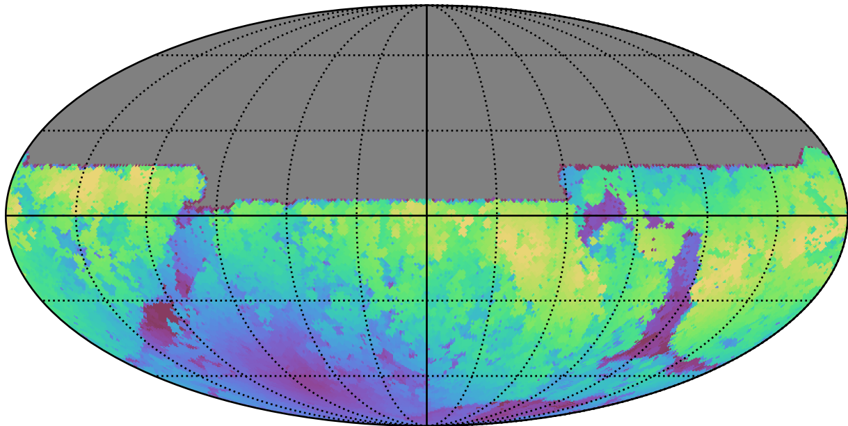
noroll_mjdp270_v3.4_10yrs All sky y band: Max moonDistance
