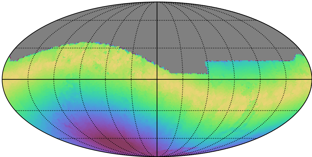
noroll_mjdp270_v3.4_10yrs All sky i band: Max moonDistance
