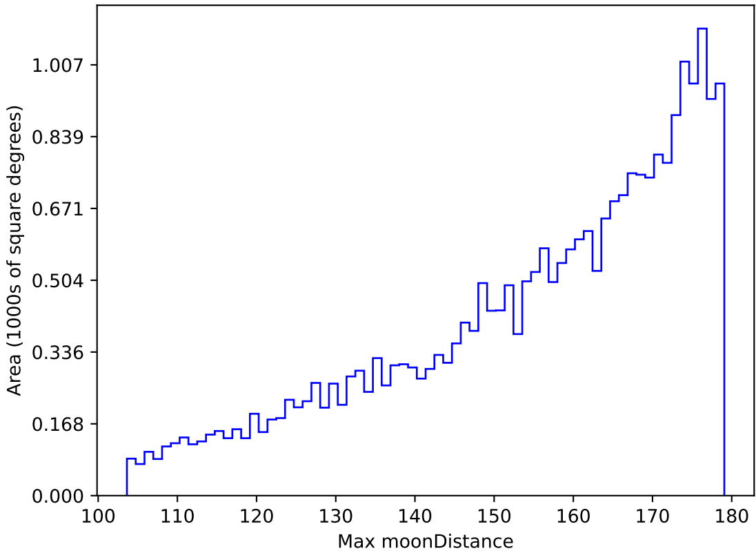
noroll_mjdp270_v3.4_10yrs All sky g band: Max moonDistance
