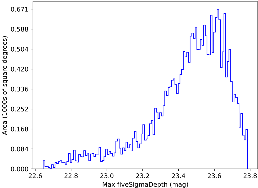
noroll_mjdp270_v3.4_10yrs Yr 1 z band: Max fiveSigmaDepth
