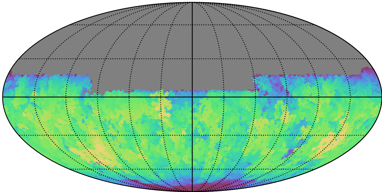
noroll_mjdp270_v3.4_10yrs Yr 1 y band: Max fiveSigmaDepth
