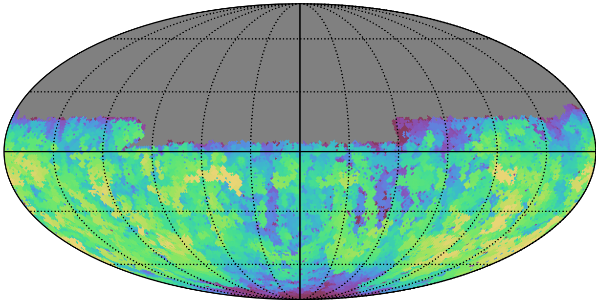
noroll_mjdp270_v3.4_10yrs Yr 1 u band: Max fiveSigmaDepth
