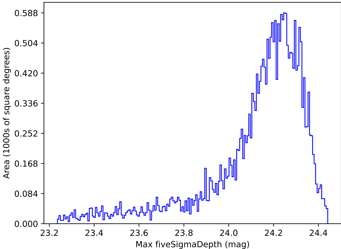
noroll_mjdp270_v3.4_10yrs Yr 1 i band: Max fiveSigmaDepth
