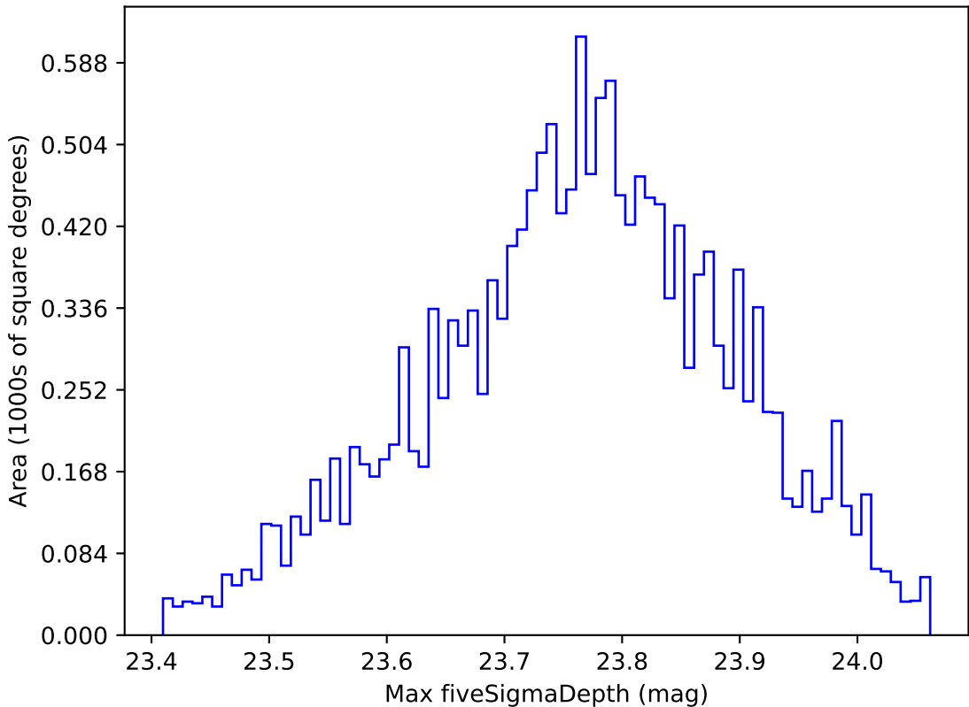
noroll_mjdp270_v3.4_10yrs WFD u band: Max fiveSigmaDepth
