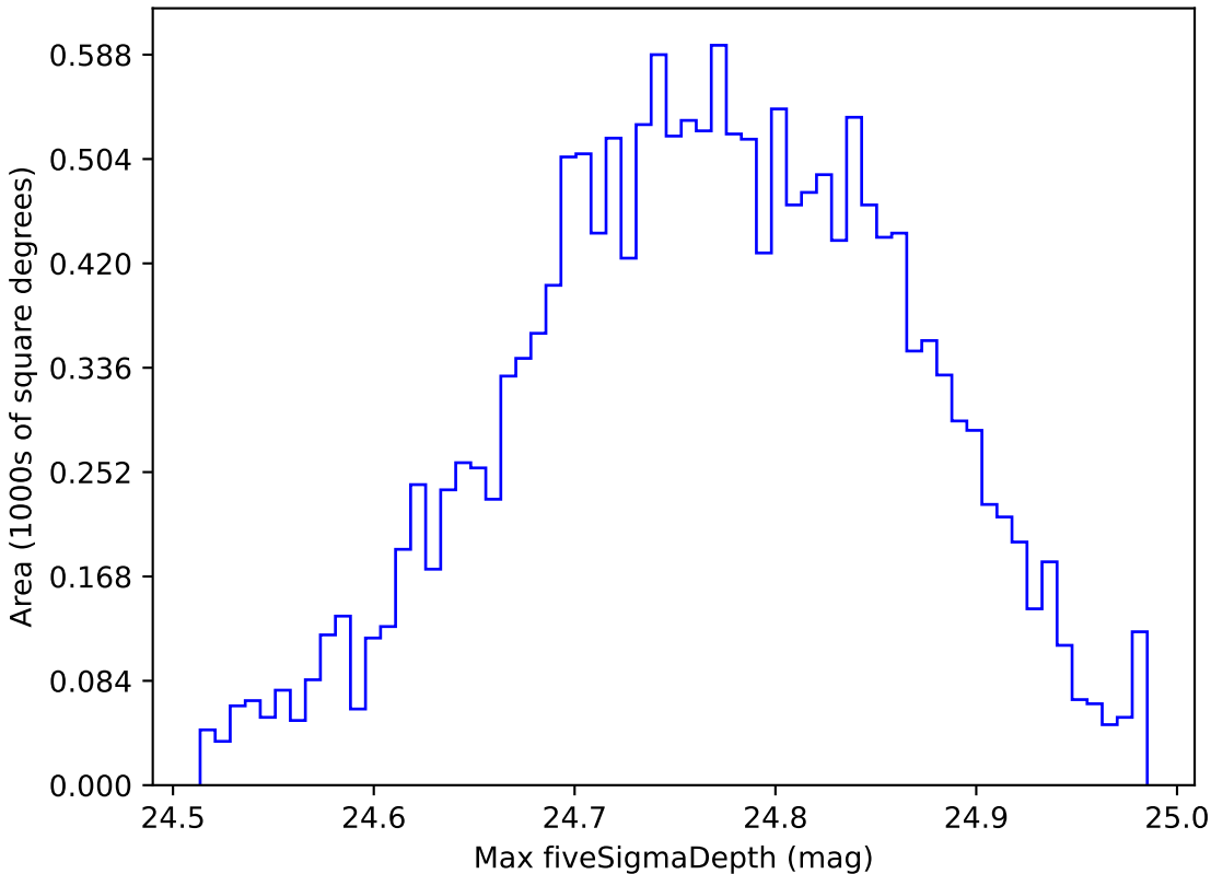
noroll_mjdp270_v3.4_10yrs WFD r band: Max fiveSigmaDepth
