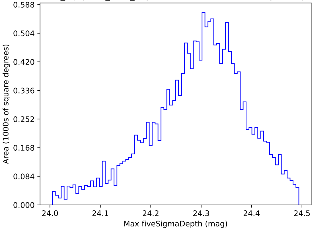
noroll_mjdp270_v3.4_10yrs WFD i band: Max fiveSigmaDepth
