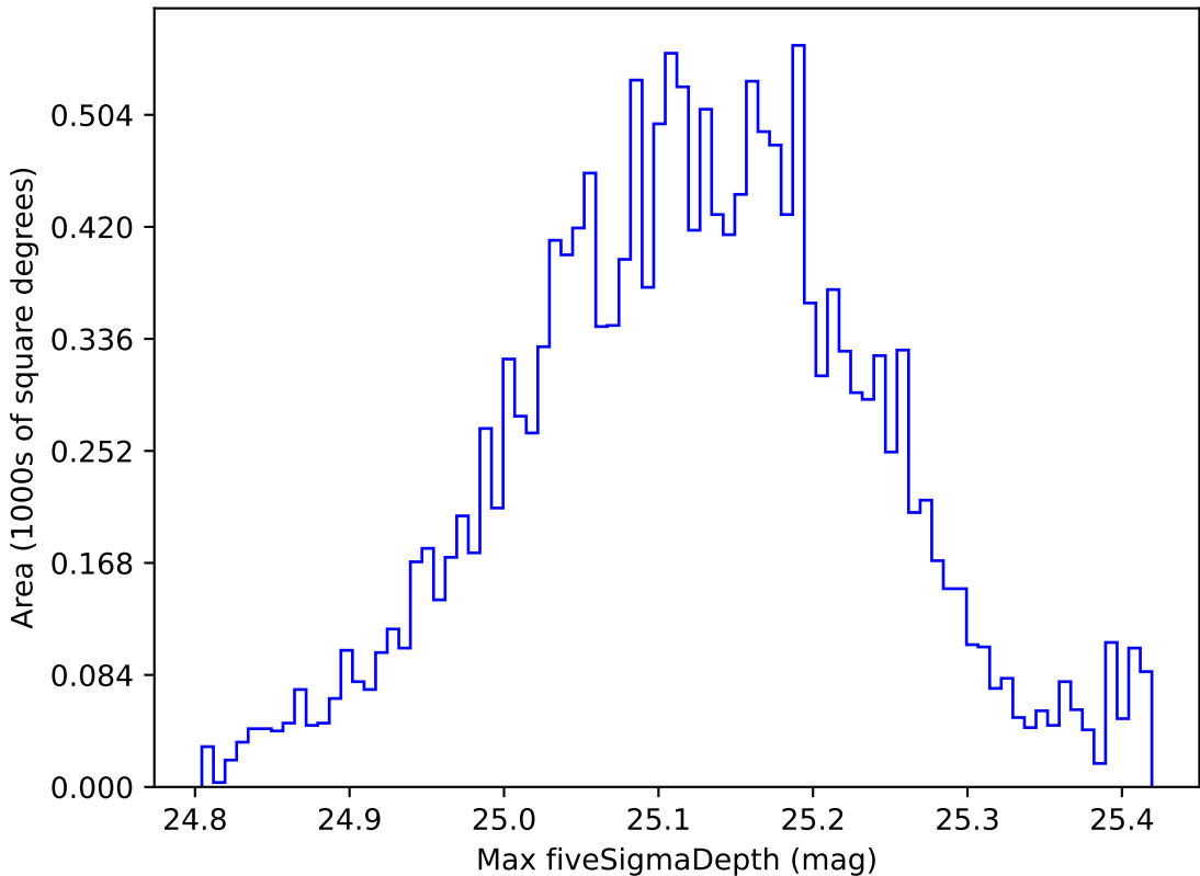
noroll_mjdp270_v3.4_10yrs WFD g band: Max fiveSigmaDepth
