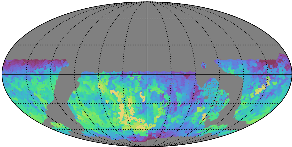
noroll_mjdp270_v3.4_10yrs WFD all bands: Max fiveSigmaDepth
