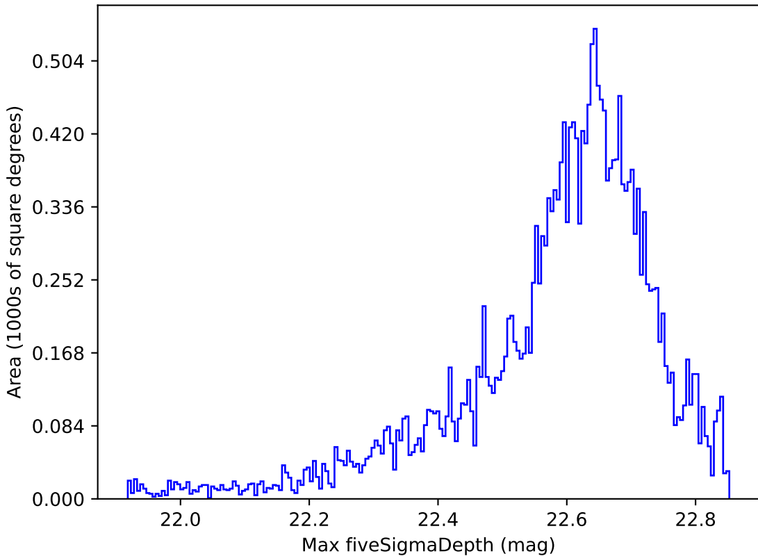
noroll_mjdp270_v3.4_10yrs All sky y band: Max fiveSigmaDepth
