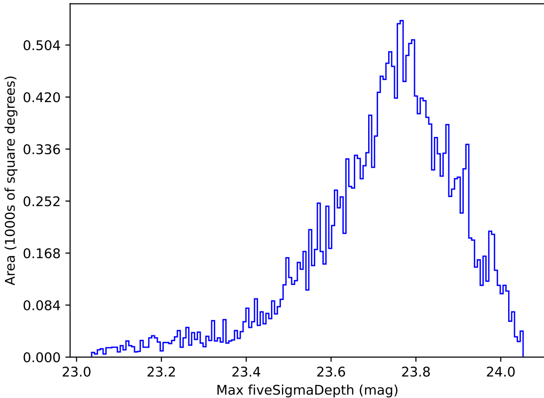
noroll_mjdp270_v3.4_10yrs All sky u band: Max fiveSigmaDepth
