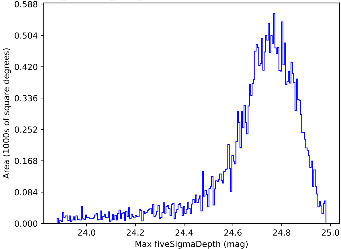
noroll_mjdp270_v3.4_10yrs All sky r band: Max fiveSigmaDepth
